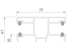
Double-sided (ALU) roller guide - RSW A939
