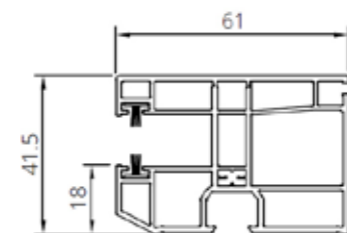
Roller guide (PVC) one-sided MINI.
