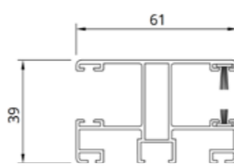
Roller guide (ALU) one-sided / two-sided
