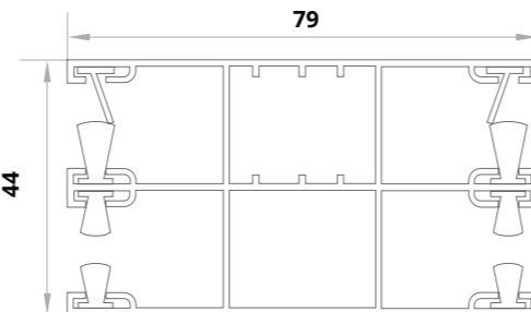
Two-sided roller guide (ALU) + MKT 87858 x2
