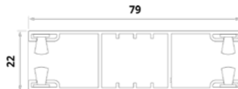
Two-sided roller guide (for H37 and H42 laths). 87858
