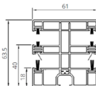
Roller guide (PVC) two-sided + MKT*.
