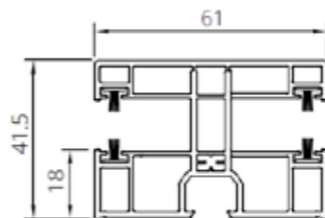
Roller guide (PVC) two-sided MINI.
